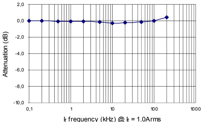
Frequency Characteristic
